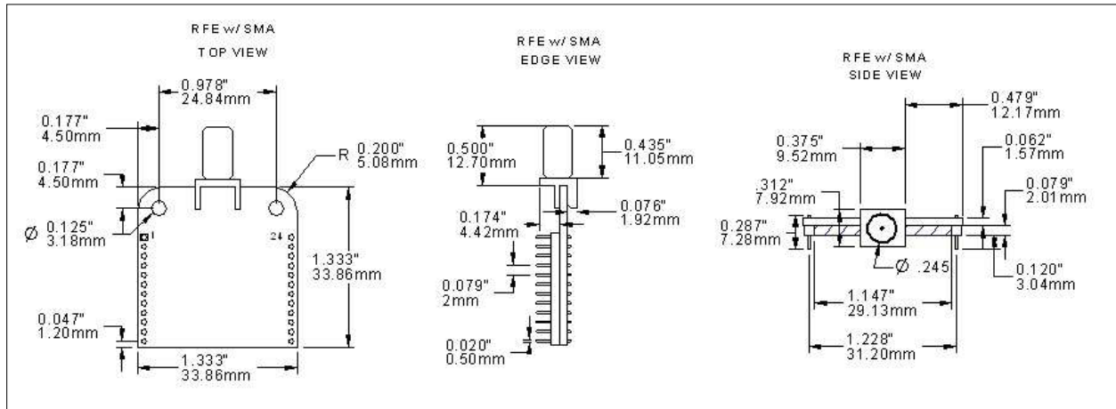
Figure 1.1 Mechanical drawings of the RF200PD1 Module
