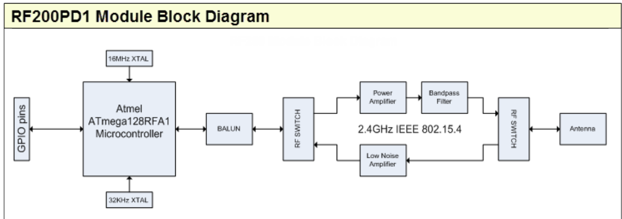
Figure 1.0 Block diagram showing the major subsystems comprising the RF200PD1
