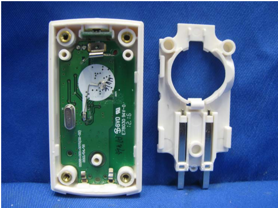
Water Sensor assembly (View 2)
