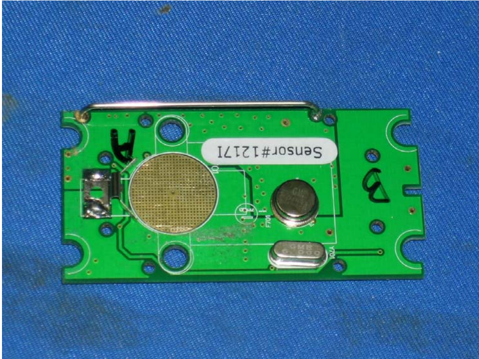
Panic Button Main PCB solder side
