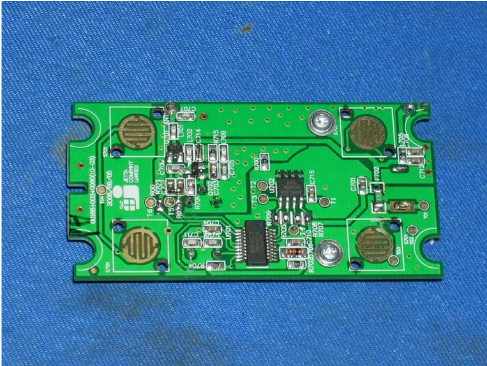
Panic Button Main PCB comp side
