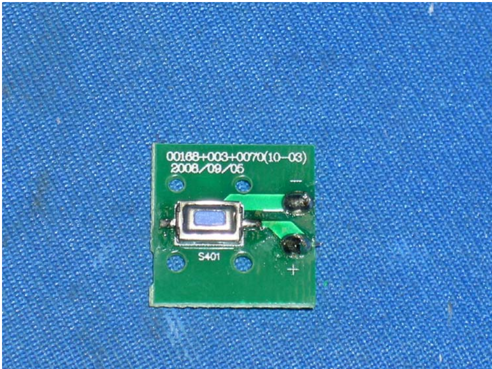
Test Button Switch PCB comp side
