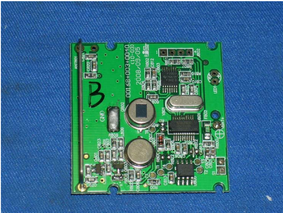
Motion Sensor Main PCB comp side
