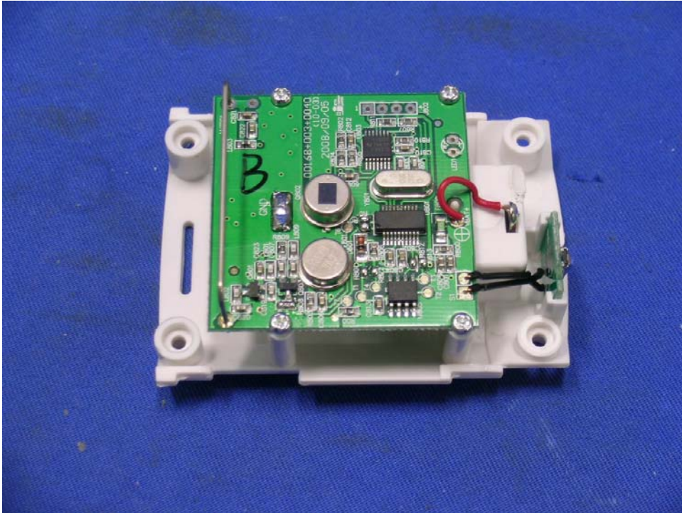
Motion Sensor assembly
