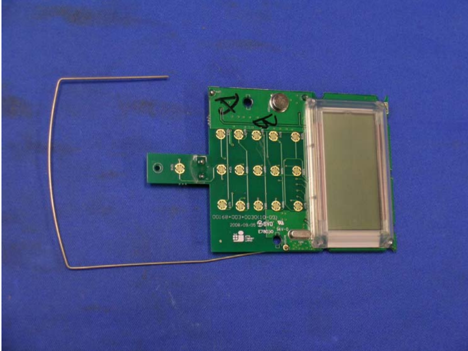
Keypad front side (View 1)
