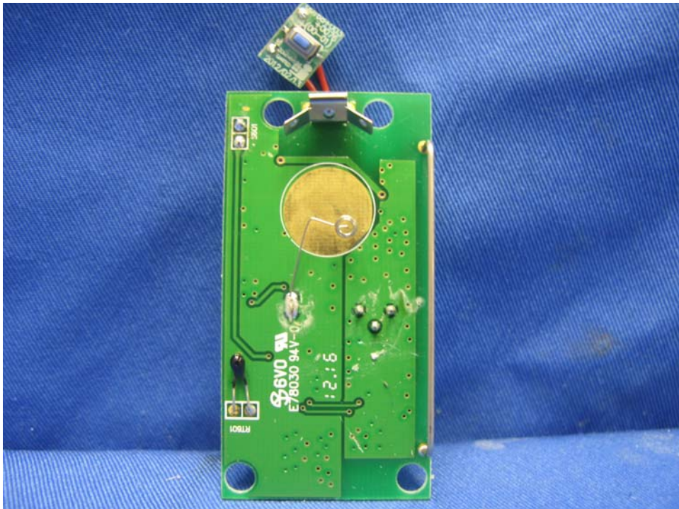
Freeze Sensor Main PCB comp side (View 2)
