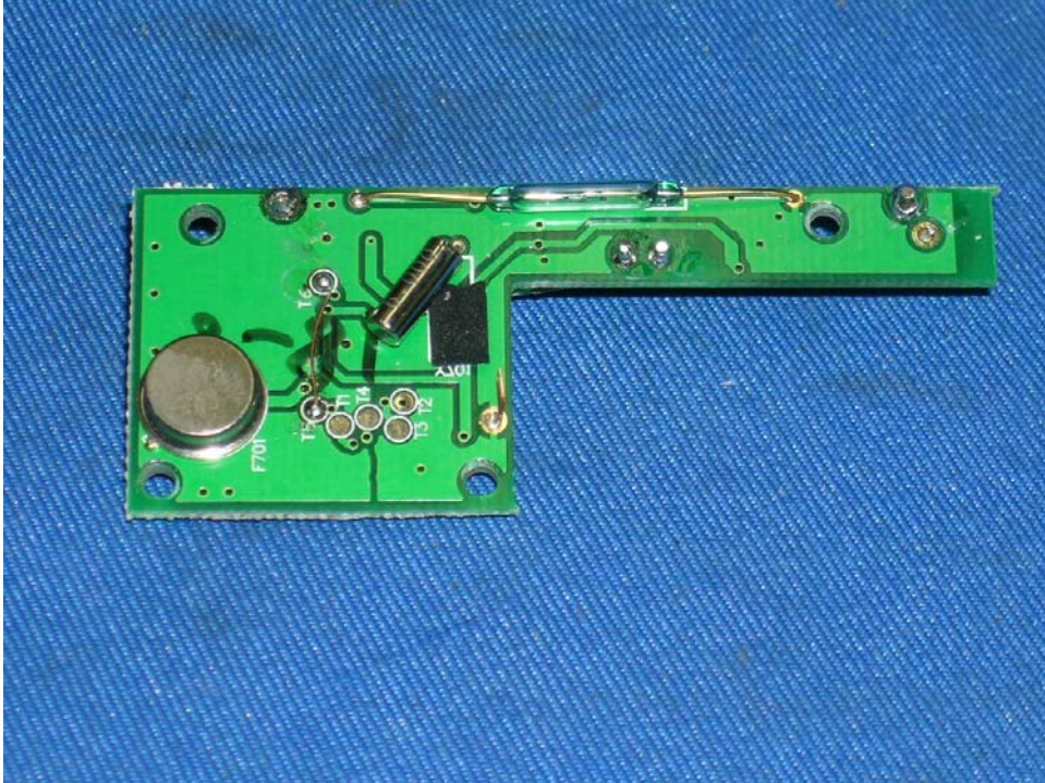
Entry Sensor Main PCB solder side
