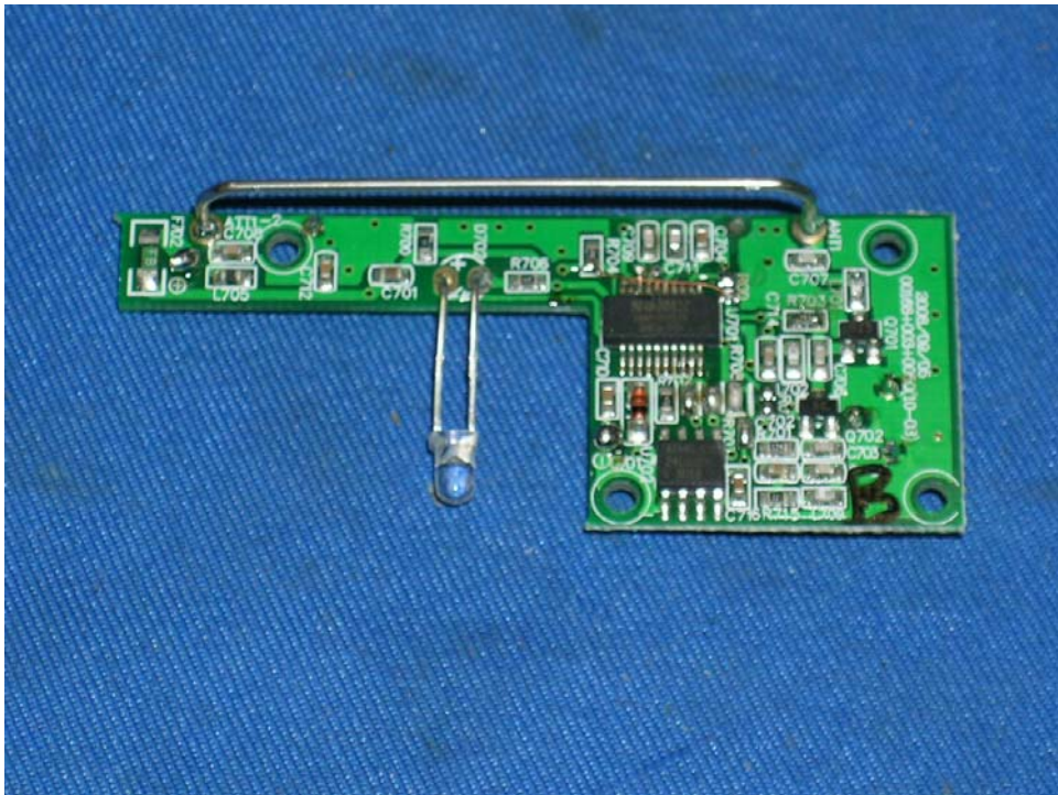
Entry Sensor Main PCB comp side
