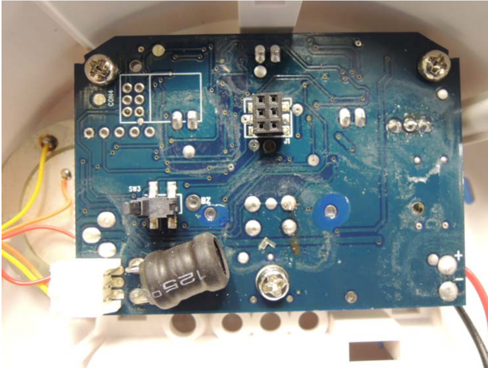
CO Detector Main PCB solder side
