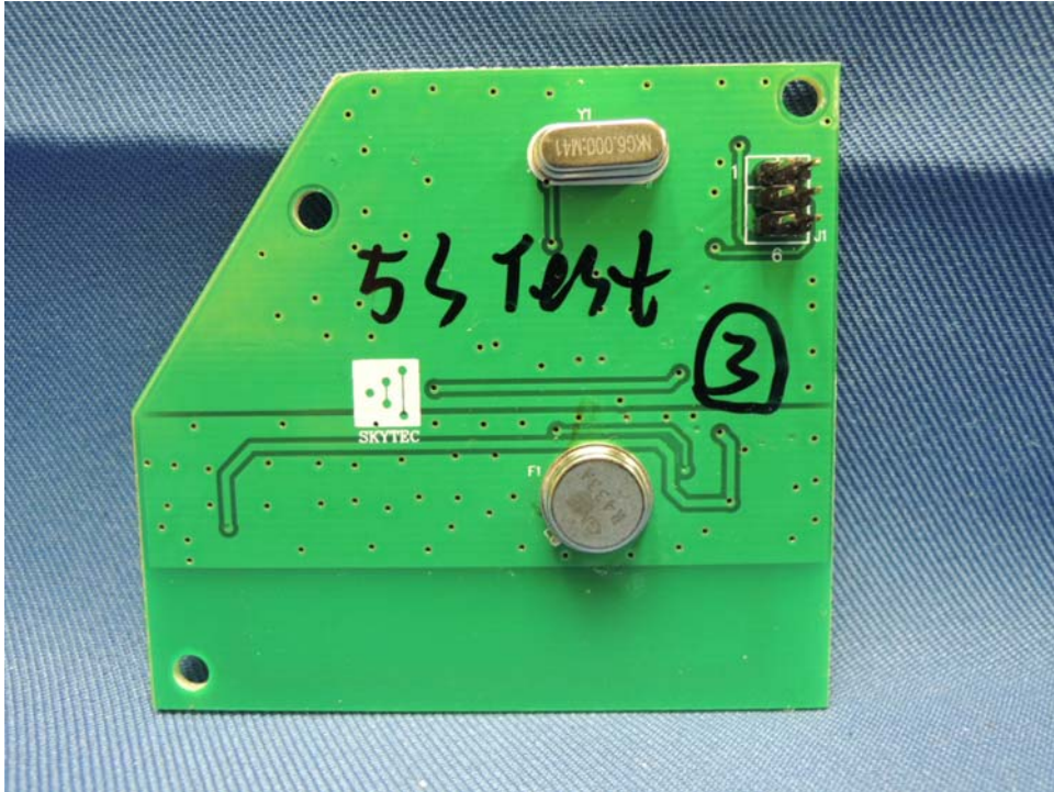
CO Detector RF Module solder side
