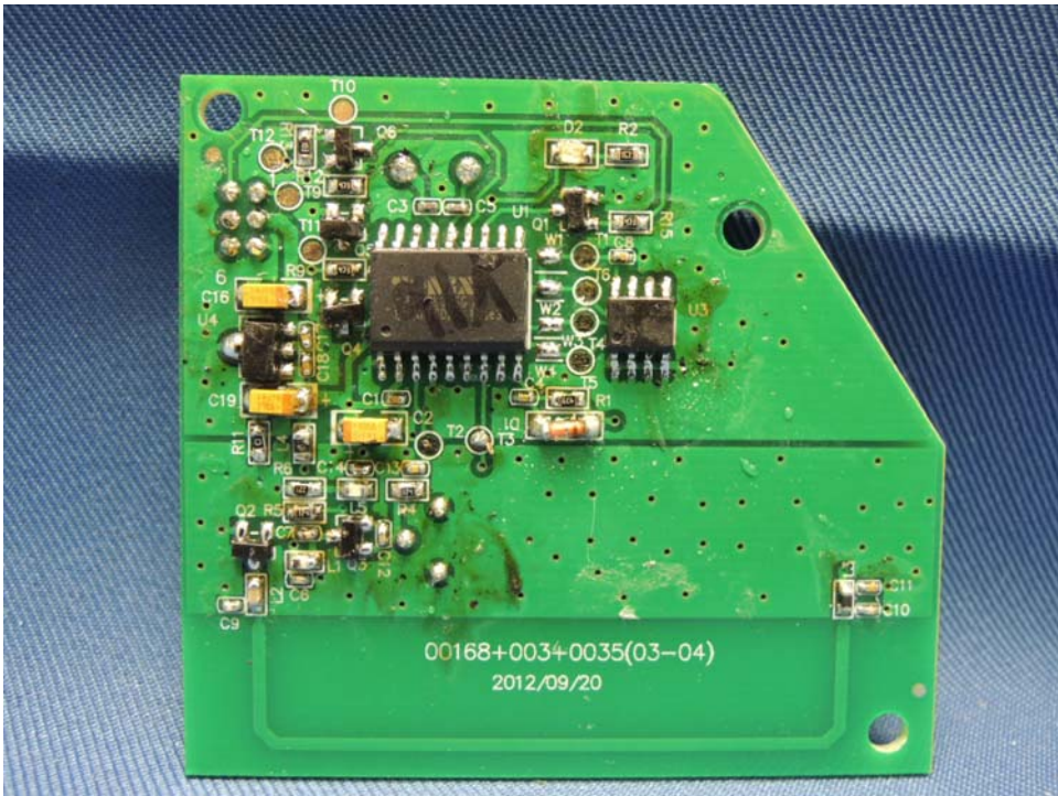
CO Detector RF Module comp side
