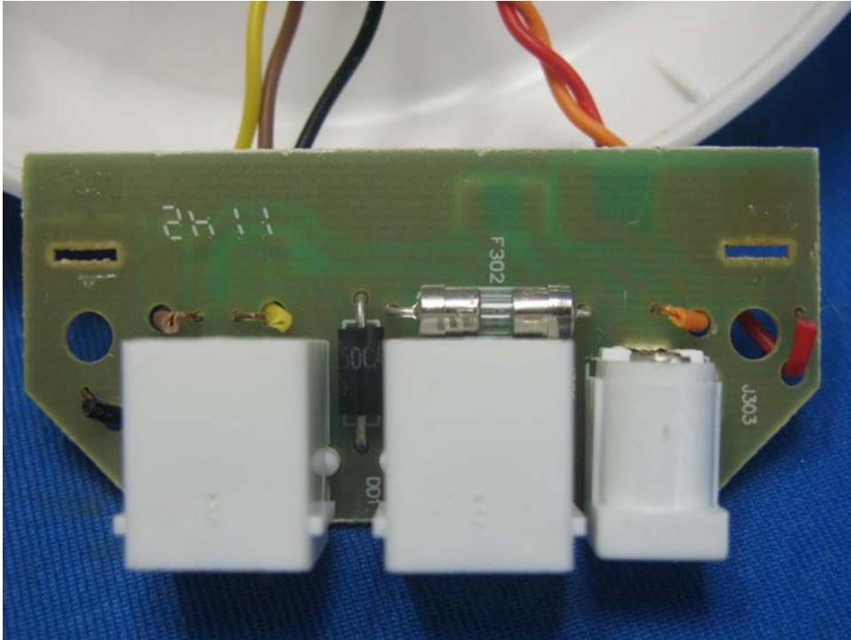
Base Station Telephone Line Jack front side
