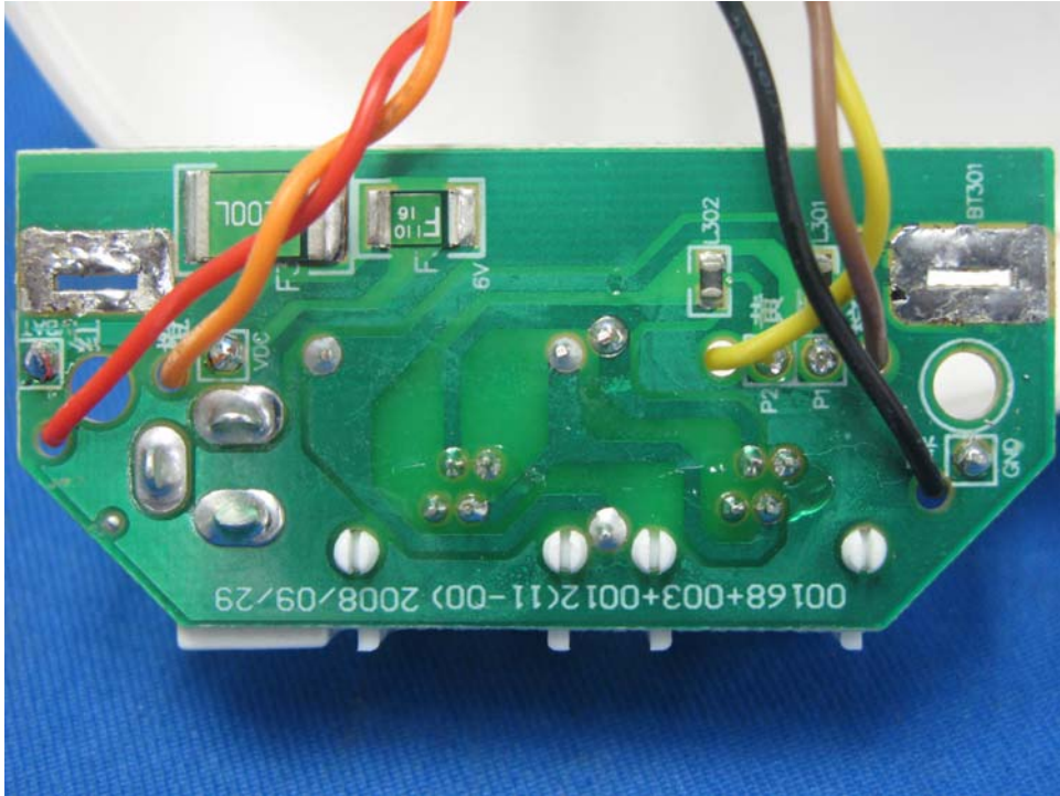
Base Station Telephone Line Jack rear side (View 2)
