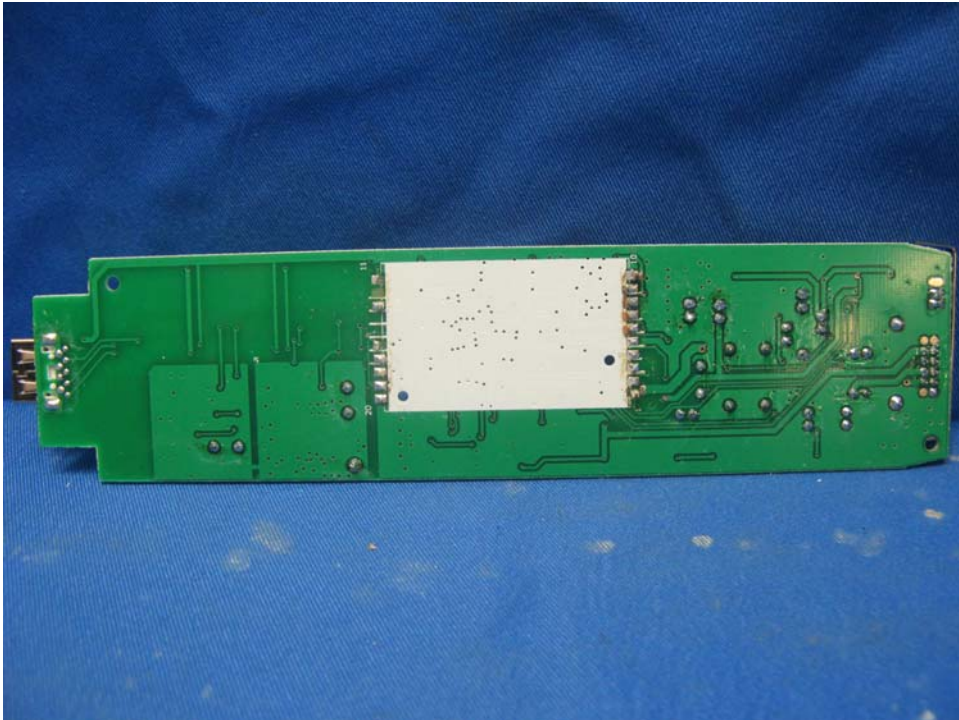
Base Station Main PCB solder side (View 2)
