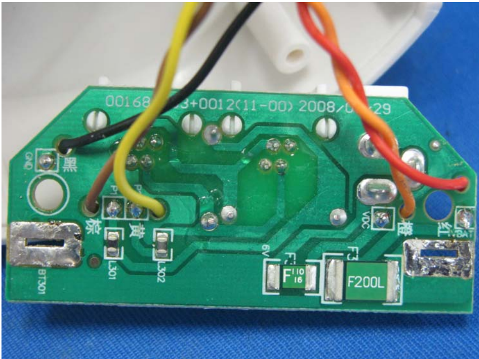
Base Station Telephone Line Jack rear side (View 1)
