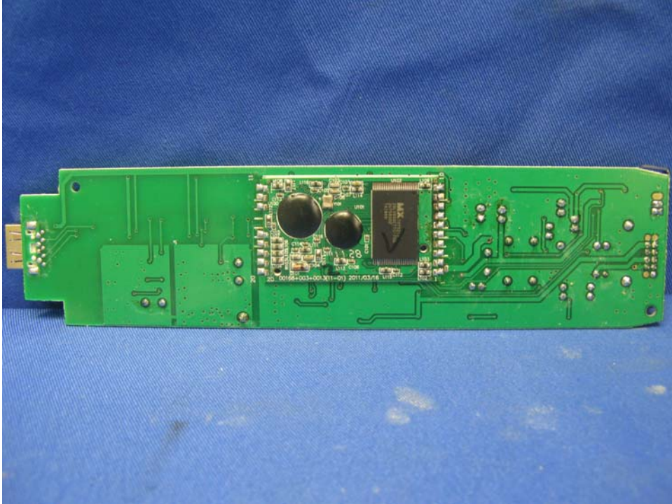
Base Station Main PCB solder side (View 1)
