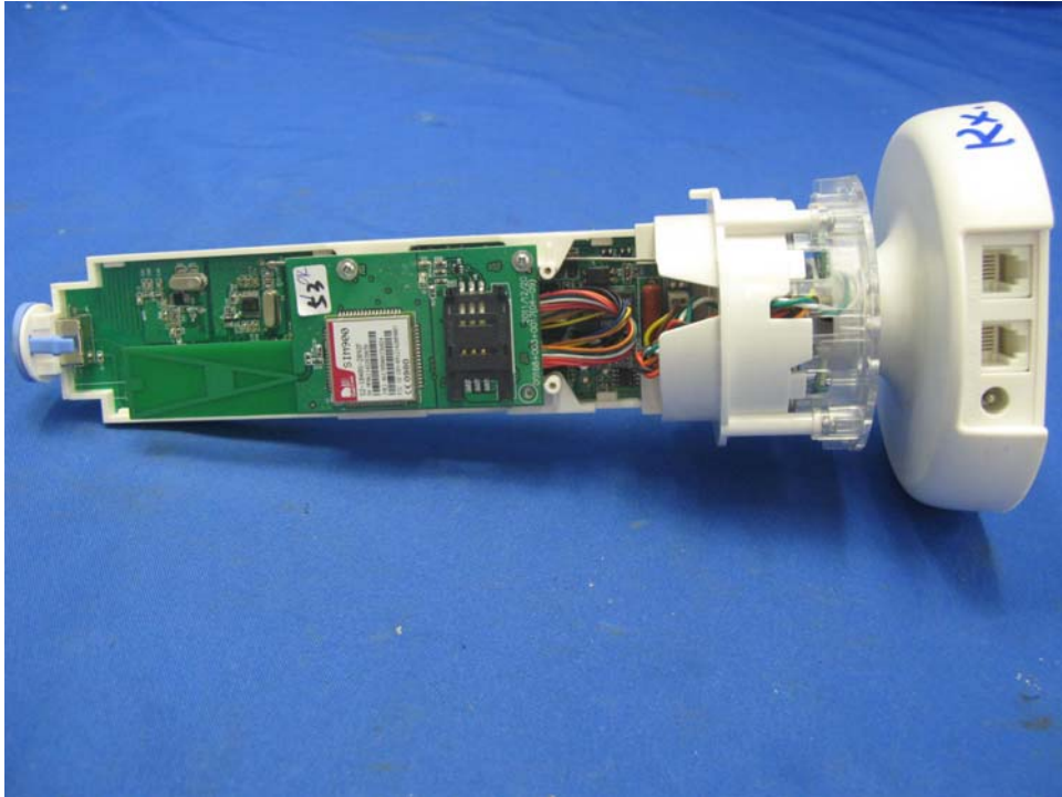
Base Station assembly
