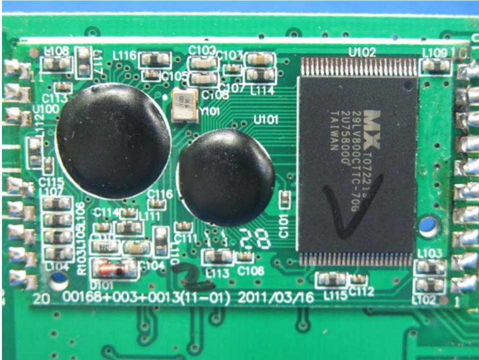
Base Station Main PCB solder side (View 3)
