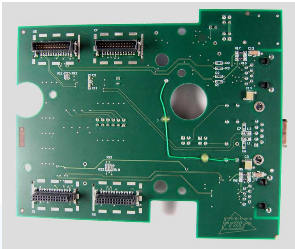
Test PCB (rear view)
