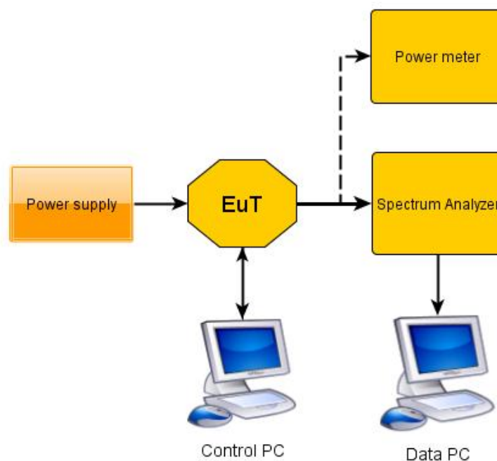
Conducted measurements
