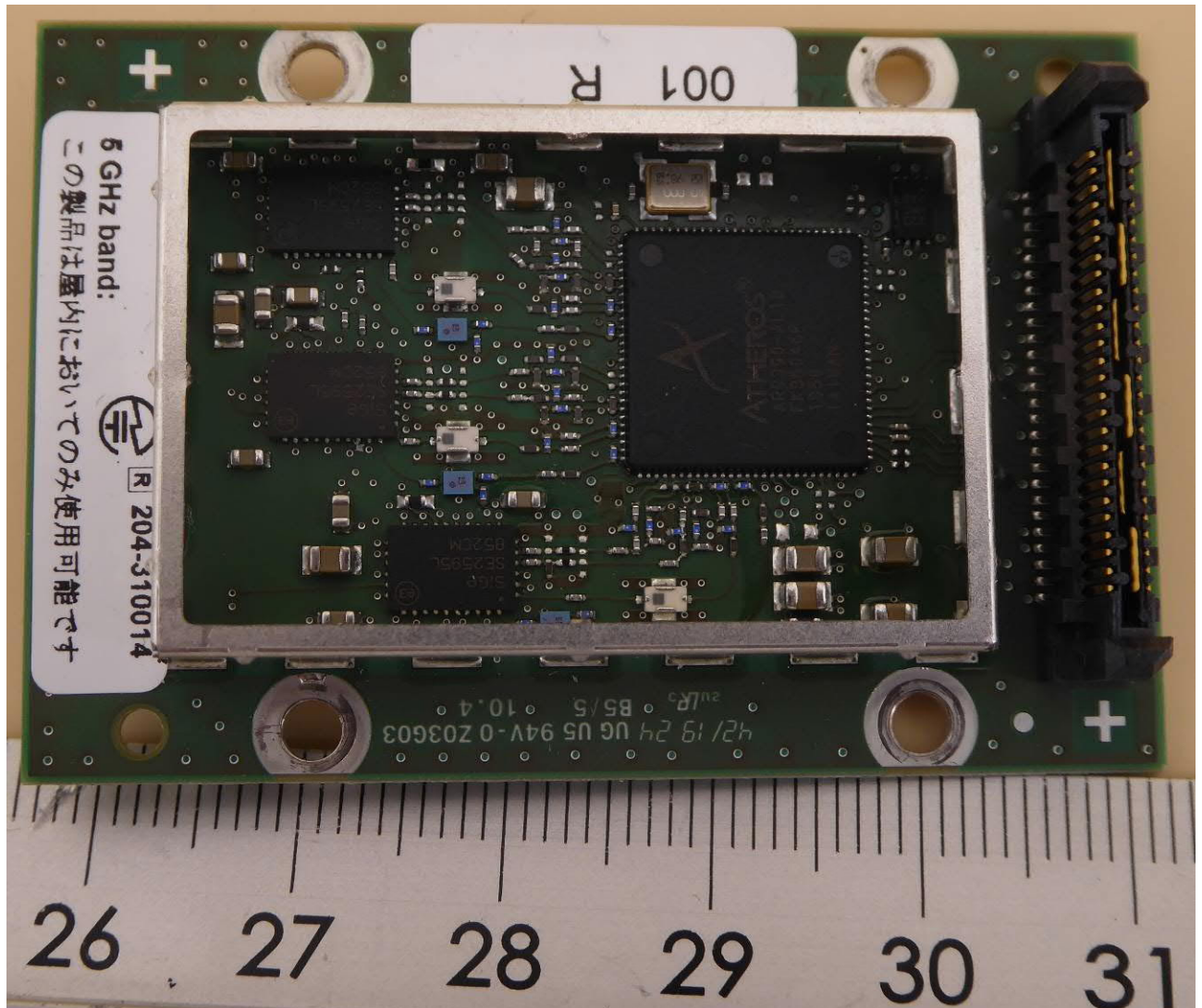
EUT without shielding – top view
