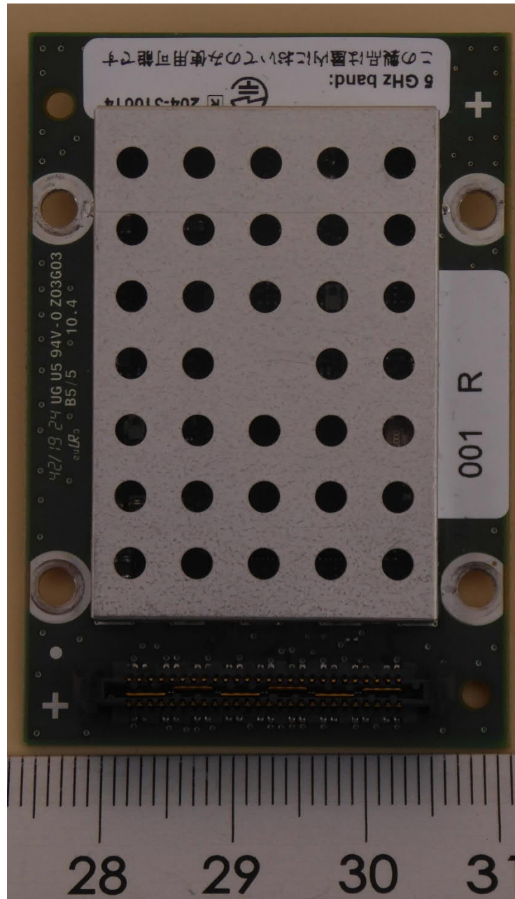
EUT with shielding – top view
