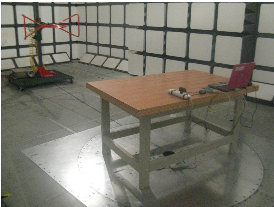
Below 1 GHz: Radiated Emissions - Rear View (Transmitting)
