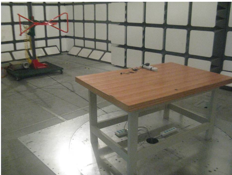
Below 1 GHz: Radiated Emissions - Rear View (Adapter Charging)
