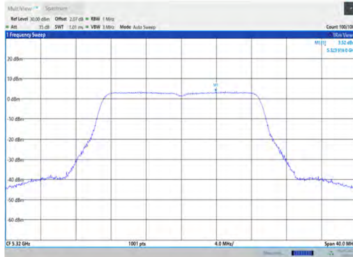
11n20SISO_Ant1_5320
