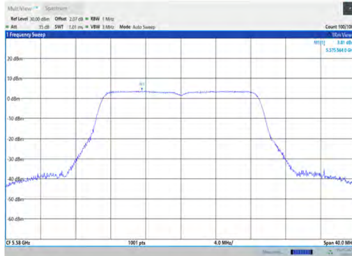
11n20SISO_Ant1_5580
