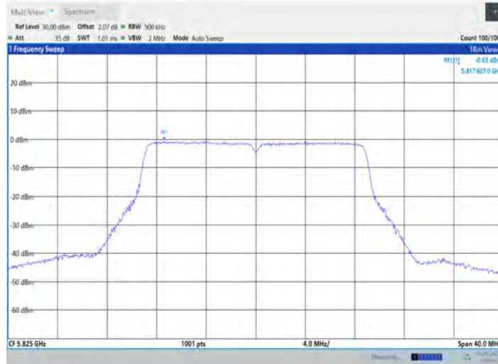
11n20SISO_Ant1_5825
