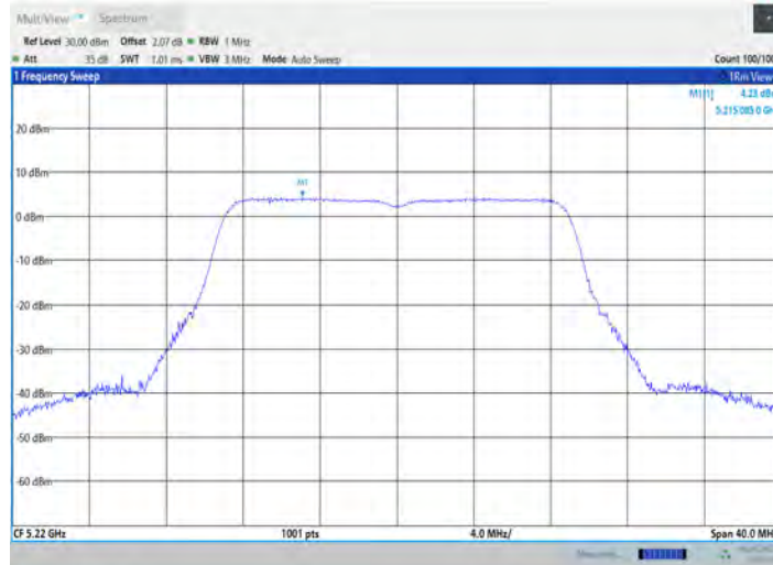
11n20SISO_Ant1_5220
