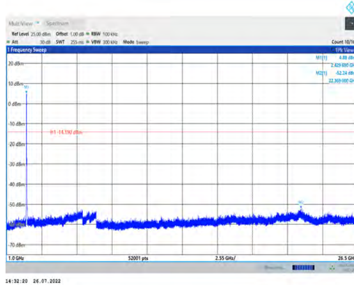
11g_Ant1_2457_0~Reference
