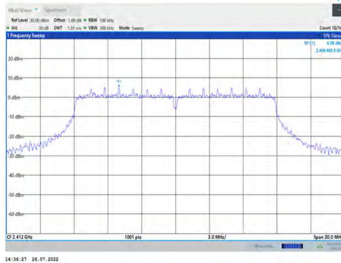
11n20SISO_Ant1_2412_0~Reference
