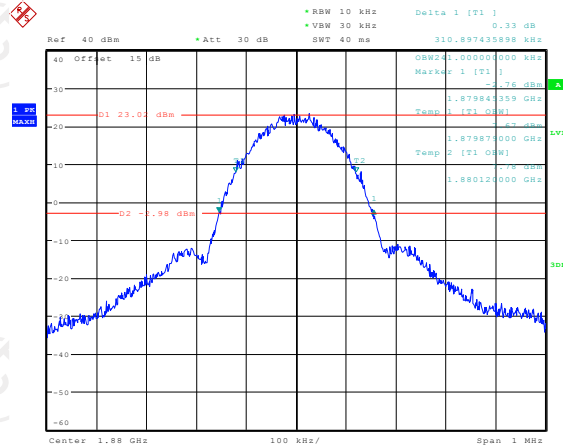
26dB&99% Occupied Bandwidth Plot on Channel 661
