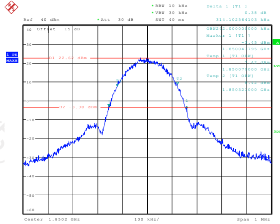
26dB&99% Occupied Bandwidth Plot on Channel 512
