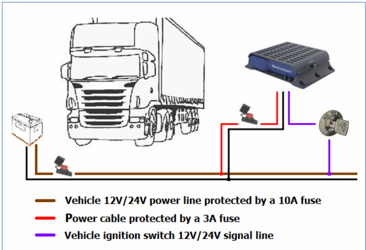
Figure 11: Electrical Installation Scheme
