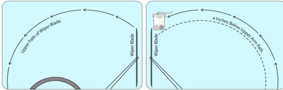
Figure 20: Micronet SmartCAM™ Double Windshield Mounting Spacing
