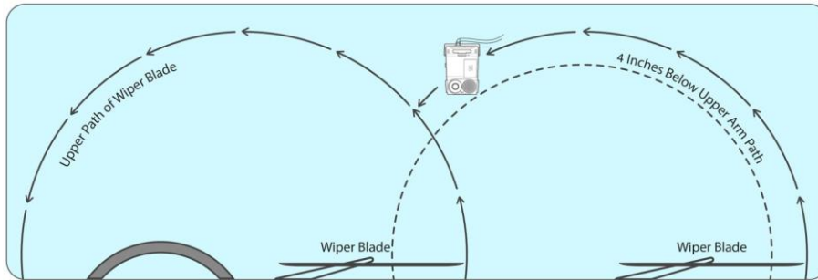
Figure 19: Micronet SmartCAM™ Single Windshield Mounting Spacing
