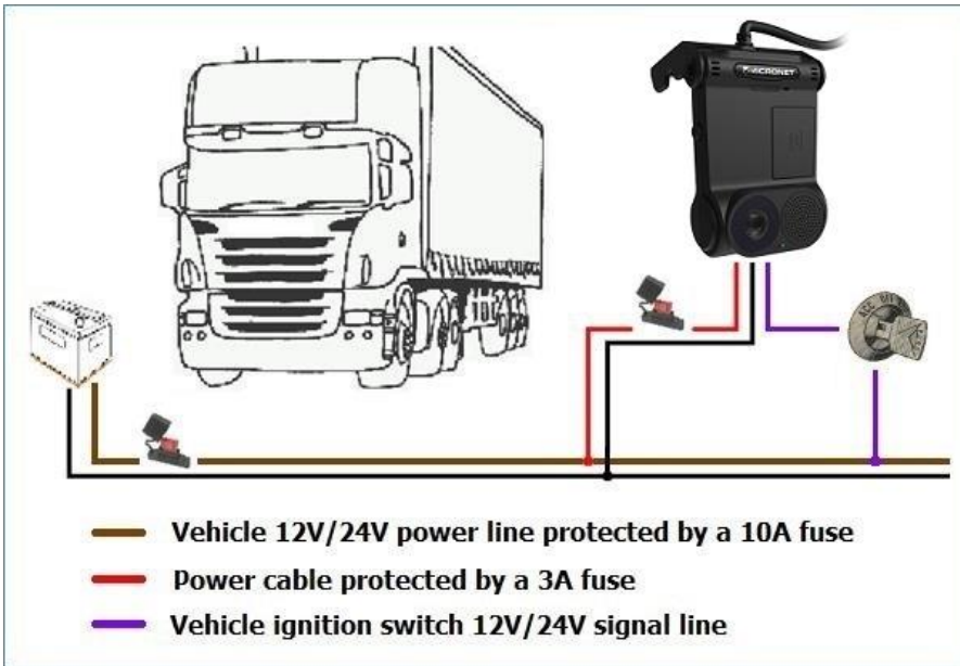
Figure 21: Electrical Installation Scheme
