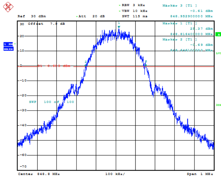
Fig.26 Channel 189- Emission Bandwidth (-26dBc BW)
