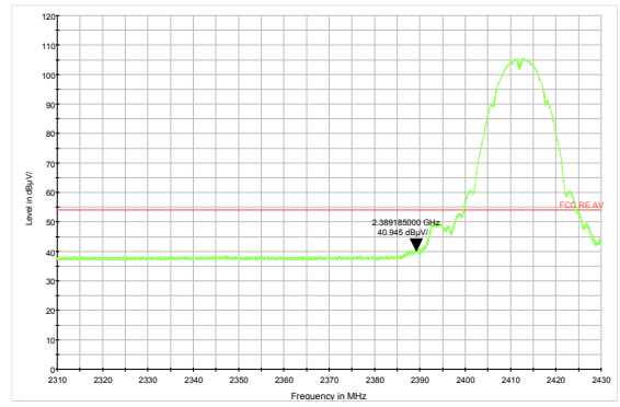
802.11b-Channel 1 Average
