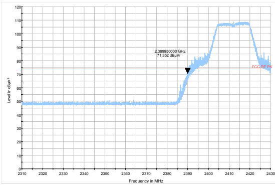
802.11g-Channel 1 Peak
