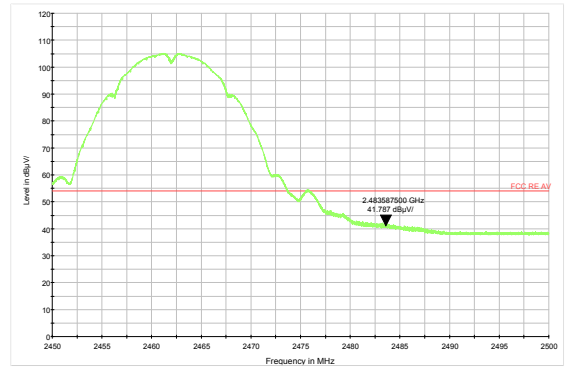
802.11b-Channel 11 Average
