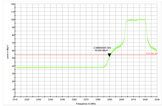
802.11g-Channel 1 Average
