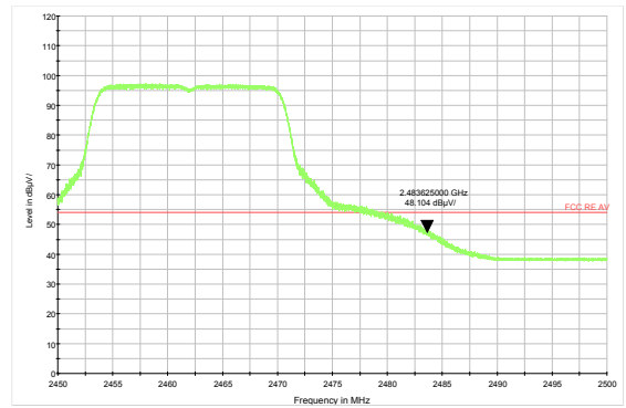
802.11g-Channel 11 Average
