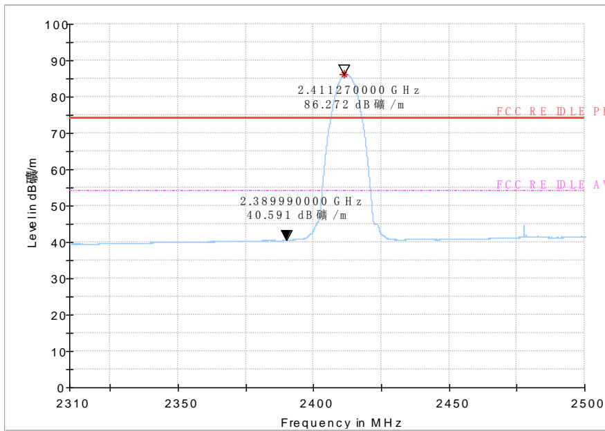
Fig 57. Bandedge: 802.11b, low channel
