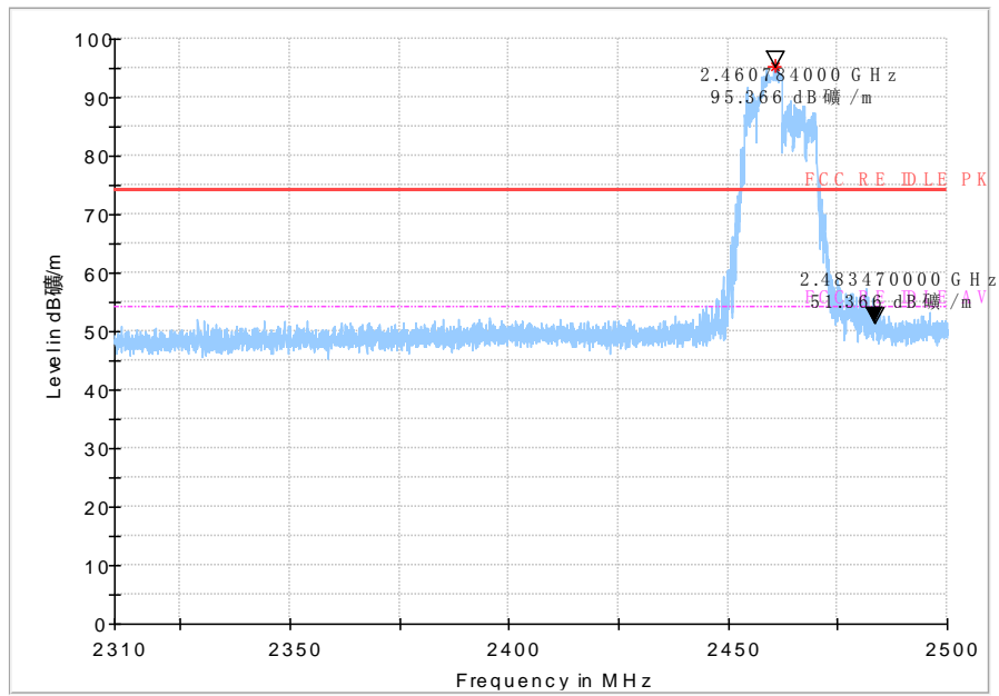
Peak detector
