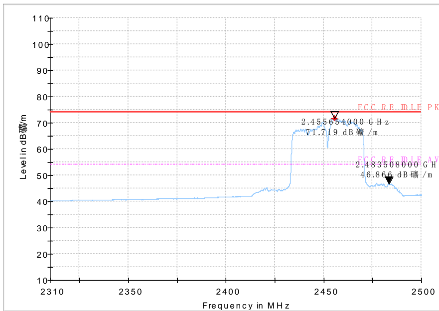
Average detector
