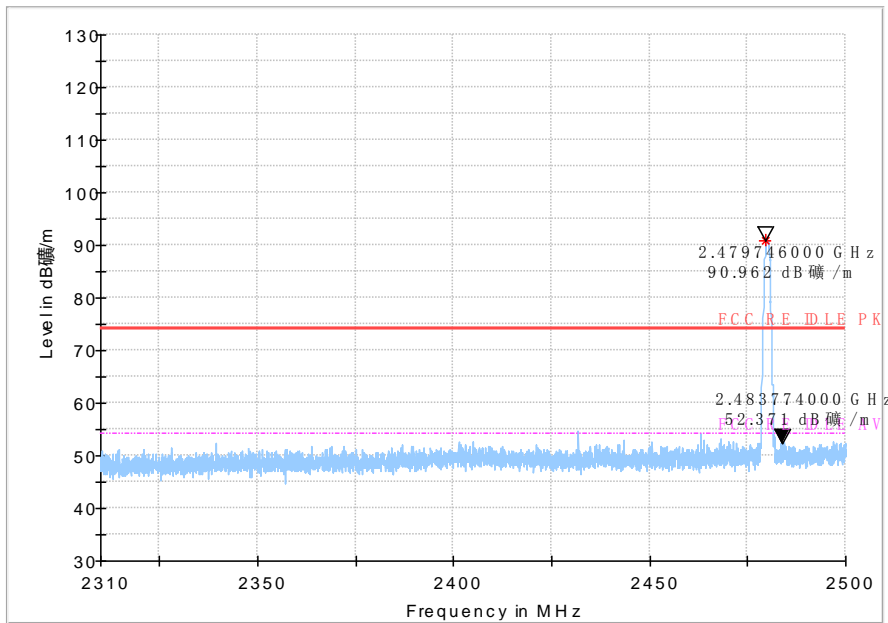
Fig.25 Bandedge:ch39
