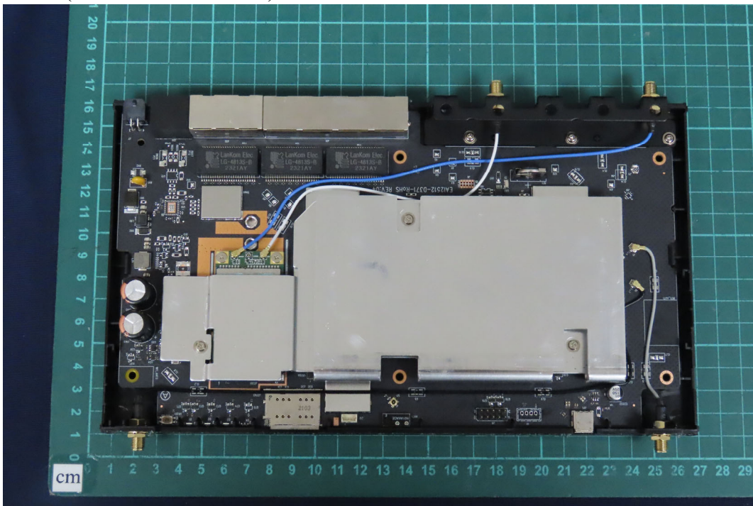
(44) EUT Photo (Model No.: B One Plus)
