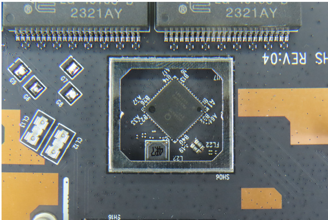
(54) EUT Photo (Model No.: B One Plus)
