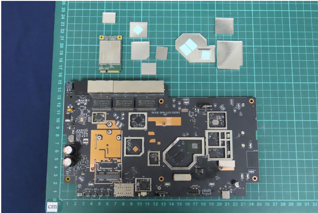
(49) EUT Photo (Model No.: B One Plus)
