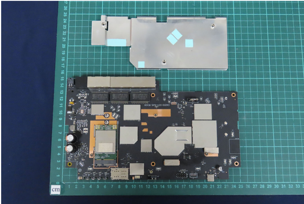
(47) EUT Photo (Model No.: B One Plus)
