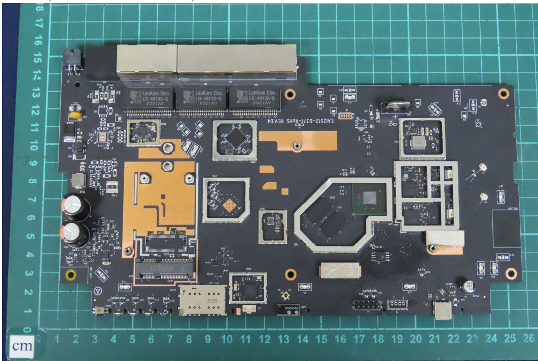
(52) EUT Photo (Model No.: B One Plus)
