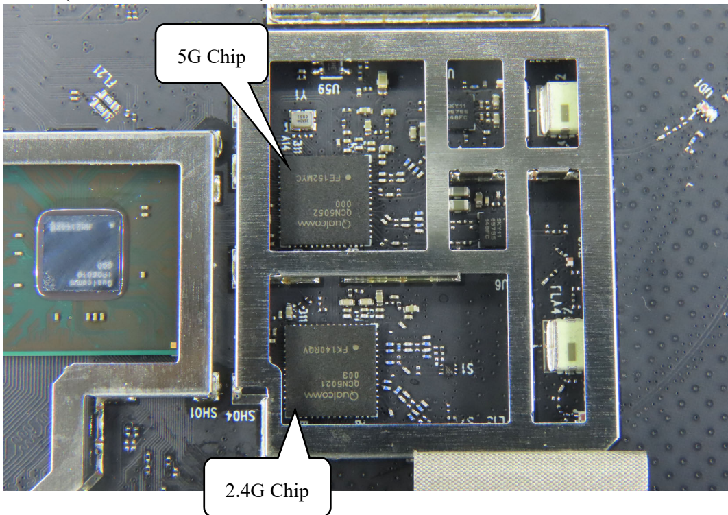
(58) EUT Photo (Model No.: B One Plus)
