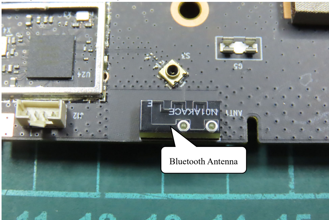
(56) EUT Photo (Model No.: B One Plus)
