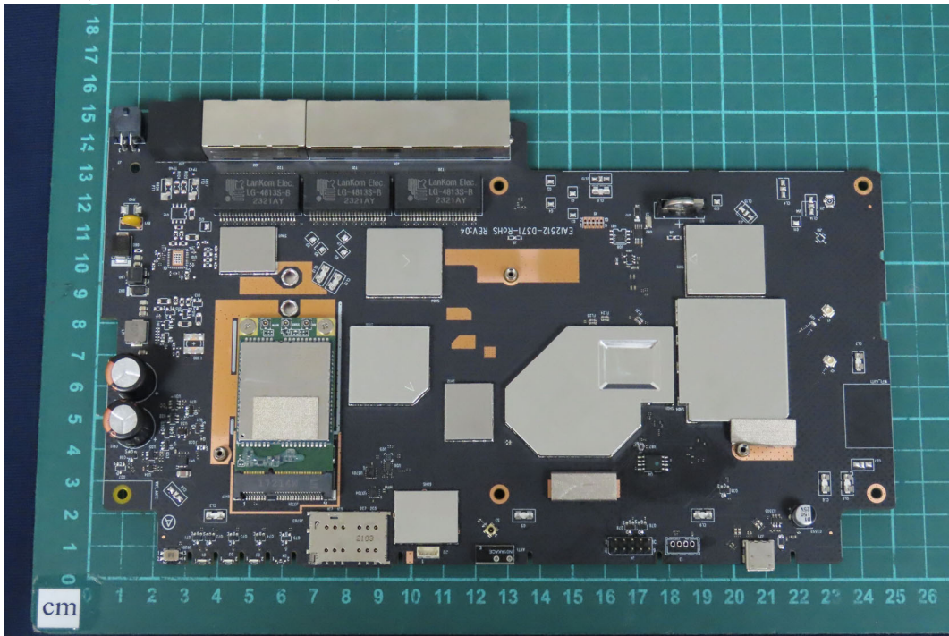
(48) EUT Photo (Model No.: B One Plus)
