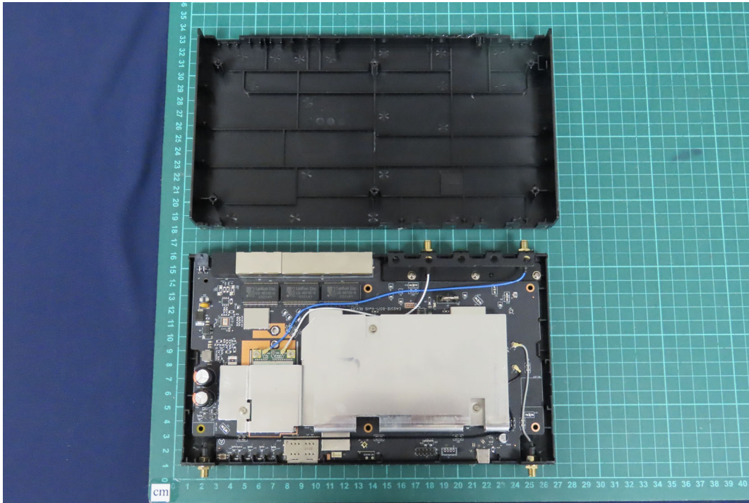
(43) EUT Photo (Model No.: B One Plus)
