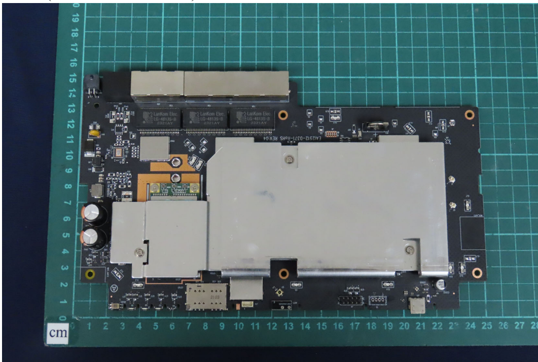
(46) EUT Photo (Model No.: B One Plus)
