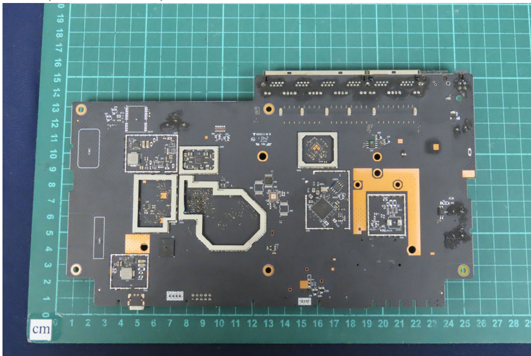
(42) EUT Photo (Model No.: B One)
