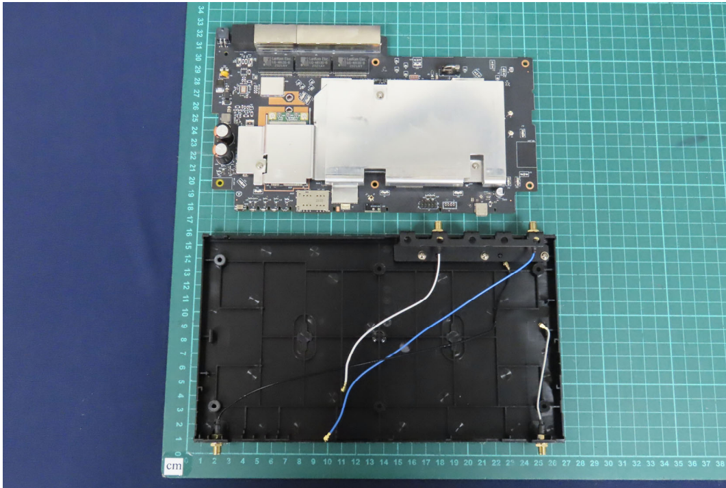
(45) EUT Photo (Model No.: B One Plus)
