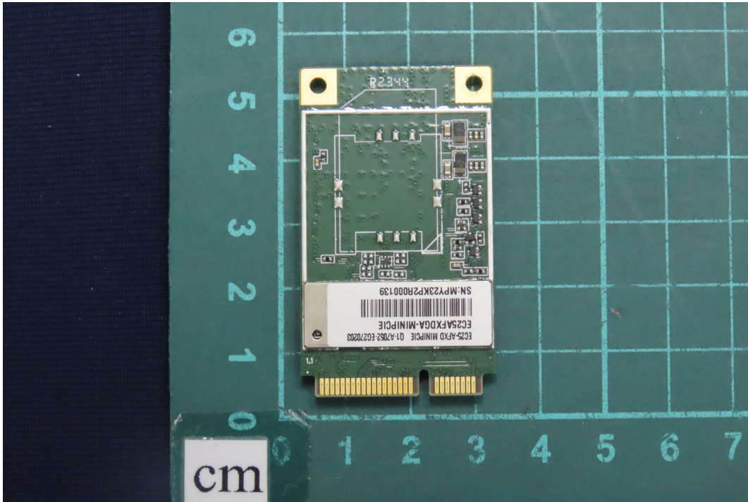
(51) EUT Photo (Model No.: B One Plus) (WWAN Module)
