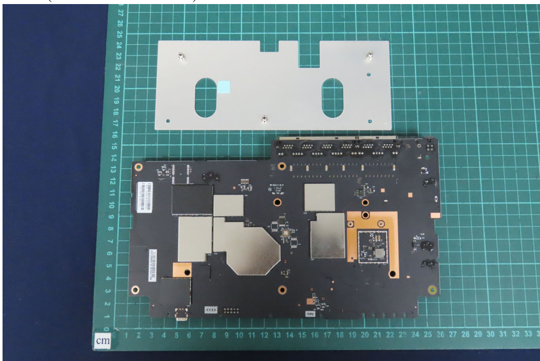
(60) EUT Photo (Model No.: B One Plus)
