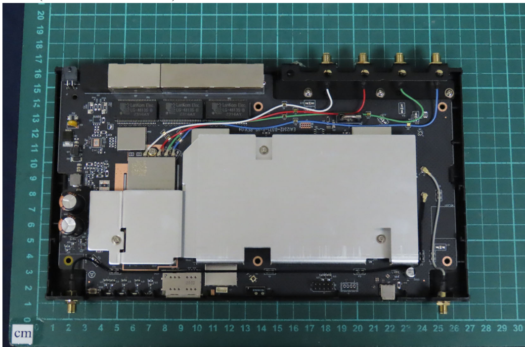
(2) EUT Photo (Model No.: B One 5G)
