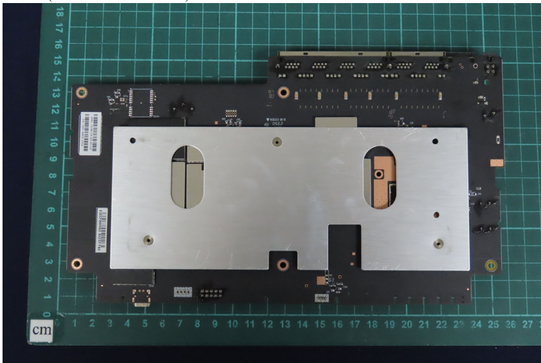
(19) EUT Photo (Model No.: B One 5G)
