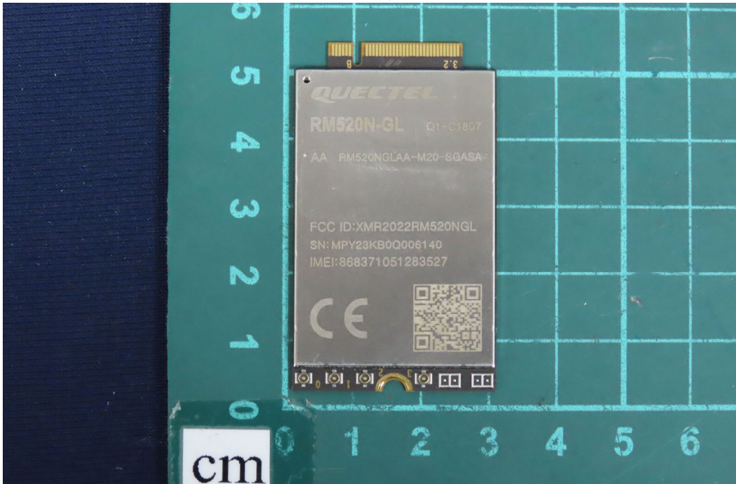
(8) EUT Photo (Model No.: B One 5G) (WWAN module)
