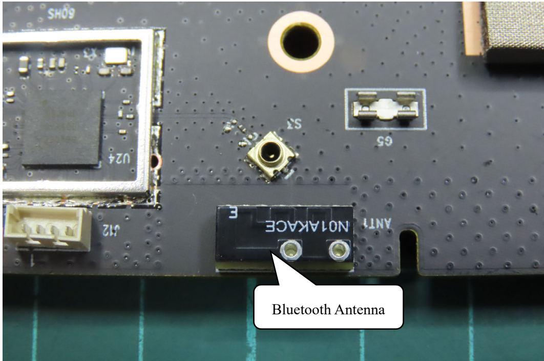
(15) EUT Photo (Model No.: B One 5G)
