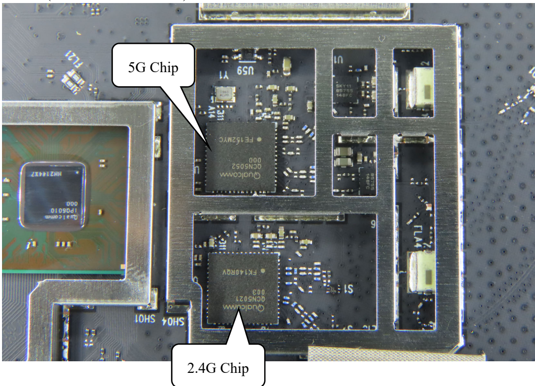
(18) EUT Photo (Model No.: B One 5G)
