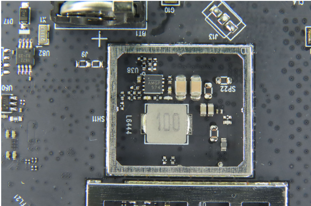
(17) EUT Photo (Model No.: B One 5G)
