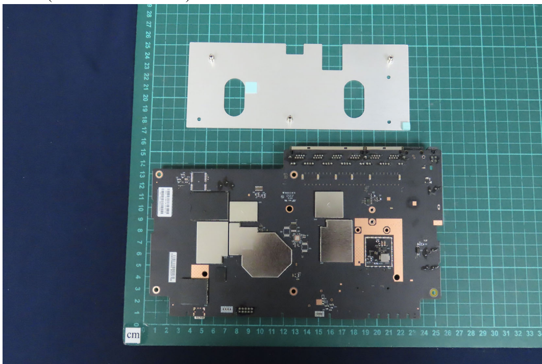
(20) EUT Photo (Model No.: B One 5G)
