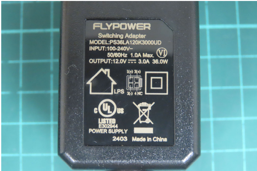
(37) EUT Photo (Adapter #2: FLYPOWER / PS36LA120K3000UD)
