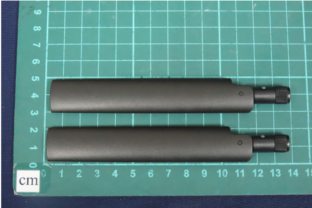
(25) EUT Photo (Model No.: B One Plus) (WWAN Antenna: INPAQ / DAM-D3-B3-N0-000-58-13)
