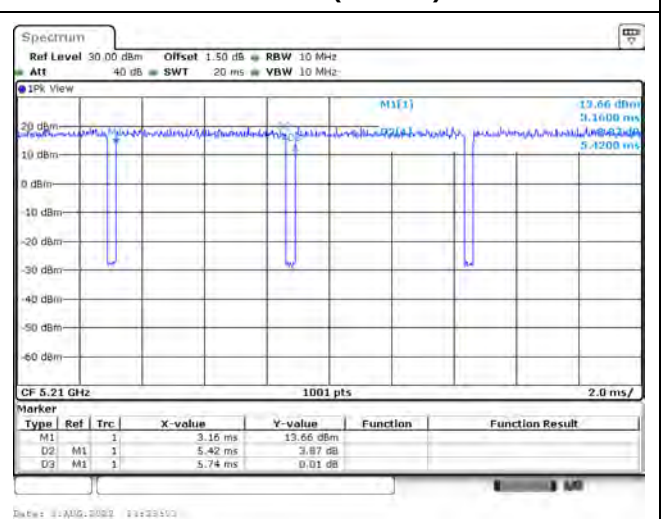
802.11ax (80 MHz)
