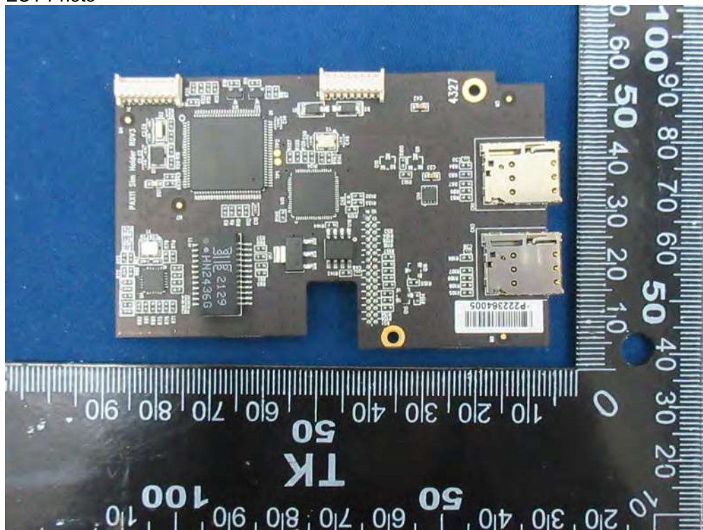
(26) EUT Photo
