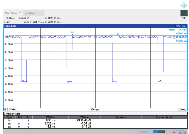
802.11ax-20 MHz
