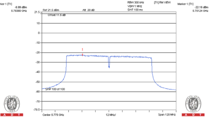
802.11ac (VHT80) – Chain 1: CH 155
