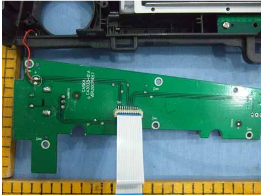
Figure 9 PCB-3 of the EUT-Back View
