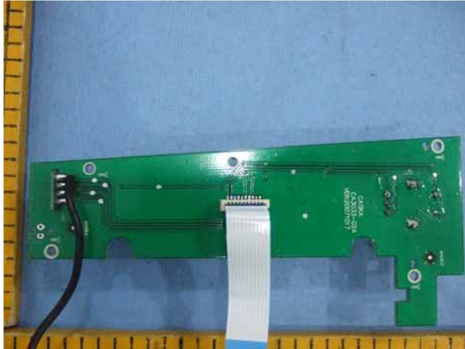
Figure 7 PCB-2 of the EUT-Back View
