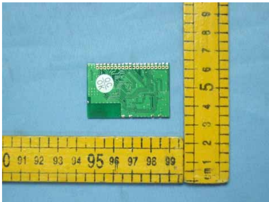
Figure 10 Bluetooth of the EUT-Bottom View
