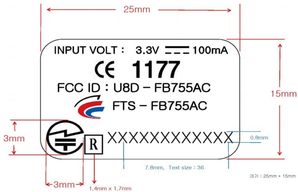
FB755AC Label
