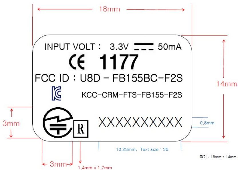
FB155BC-F2S Label
