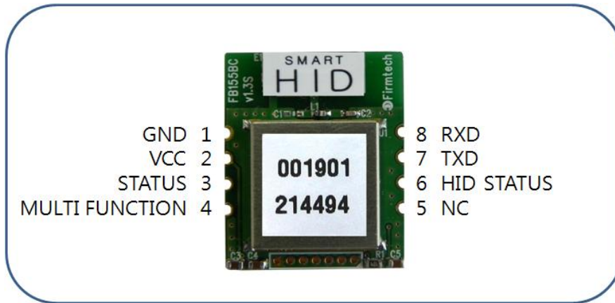
<Figure 9-2 FB155BC-F2S-HID PIN Assign>
