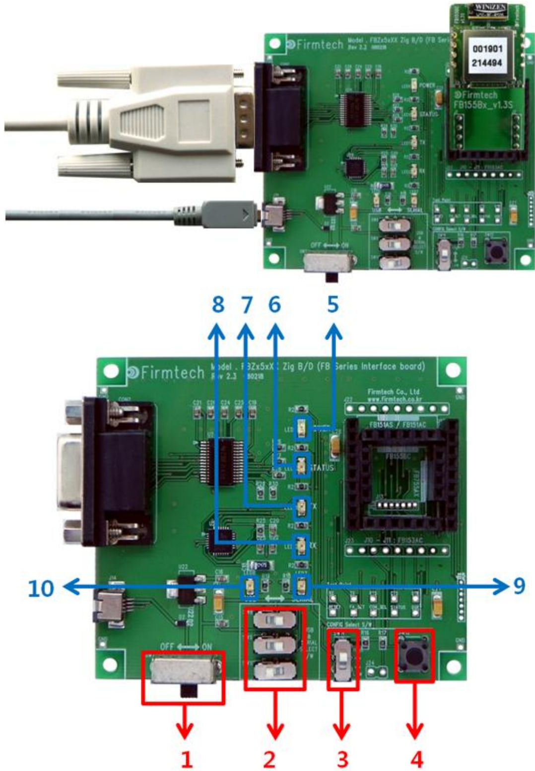
<Figure 5-1 FB155BC-F2S-SPP Interface Board(Jig Board)>
