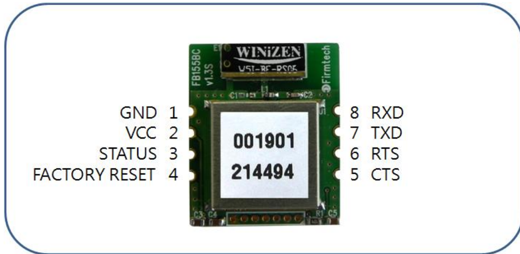
<Figure 4-2 FB155BC-F2S-SPP PIN Assign>
