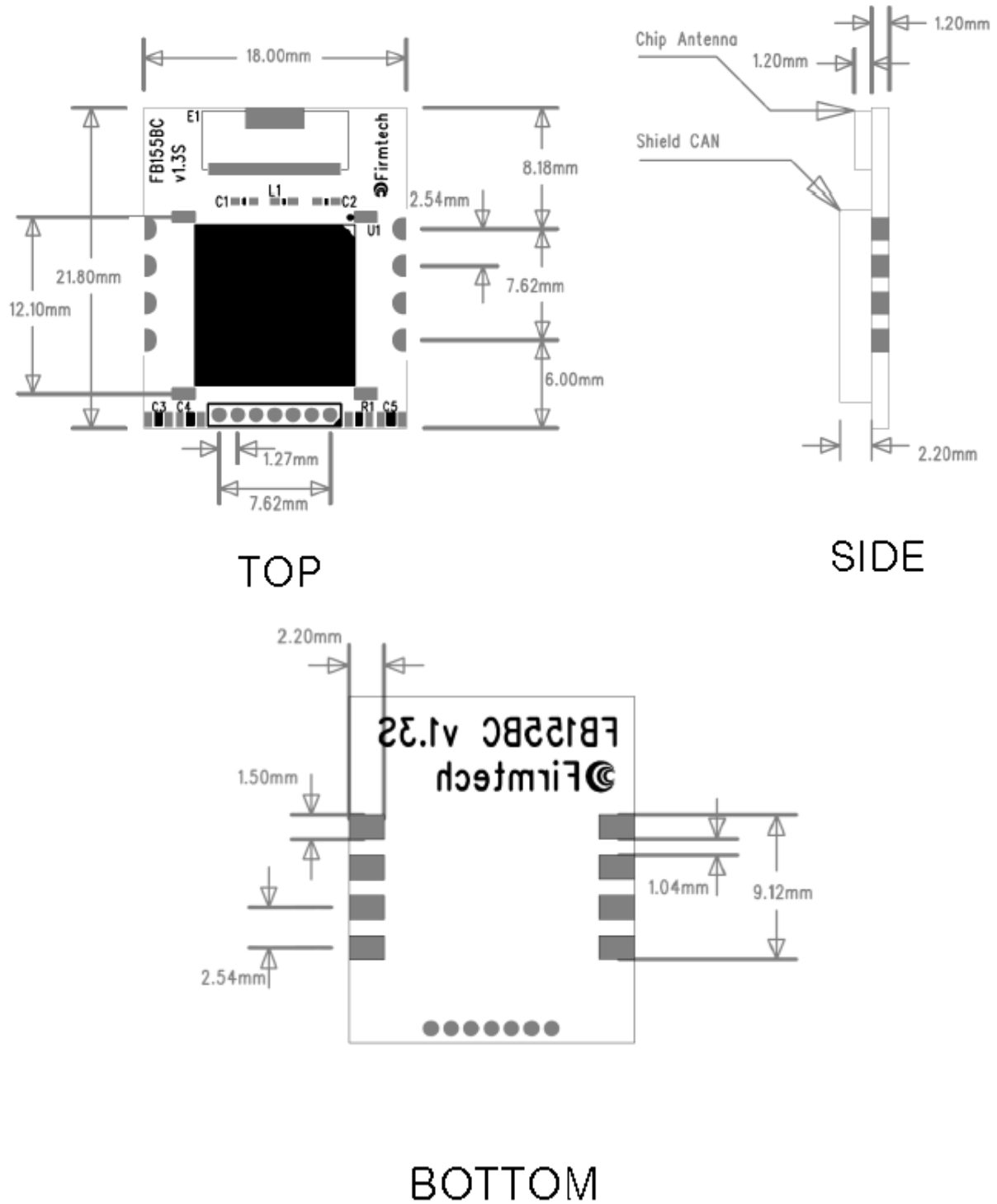
<Figure 4-1 FB155BC-F2S-SPP Dimension>
