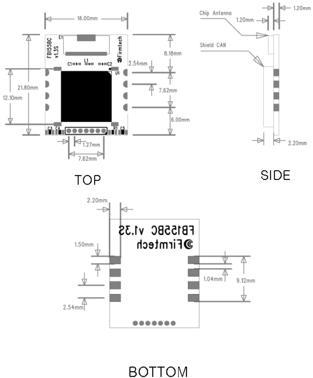
<Figure 9-1 FB155BC-F2S-HID Dimension>
