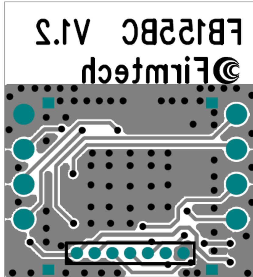
BOTTOM View
