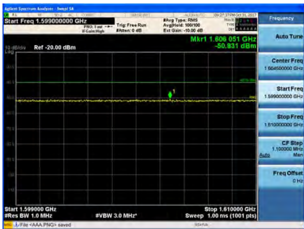
1599 MHz ~ 1610 MHz (1)
