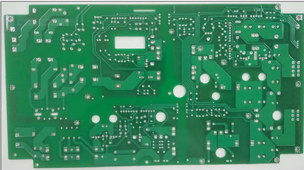
< 북미향 PS-ELITE PSU (MPS-Q1075)_MAIN PCB 밑면사진 >
