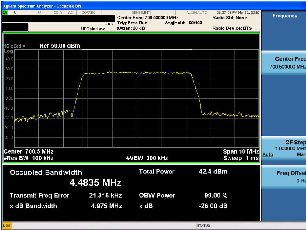
[Output Uplink Low_ AGC threshold]
