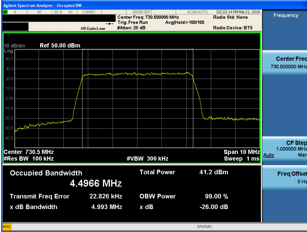
[Output Downlink Low_AGC threshold]
