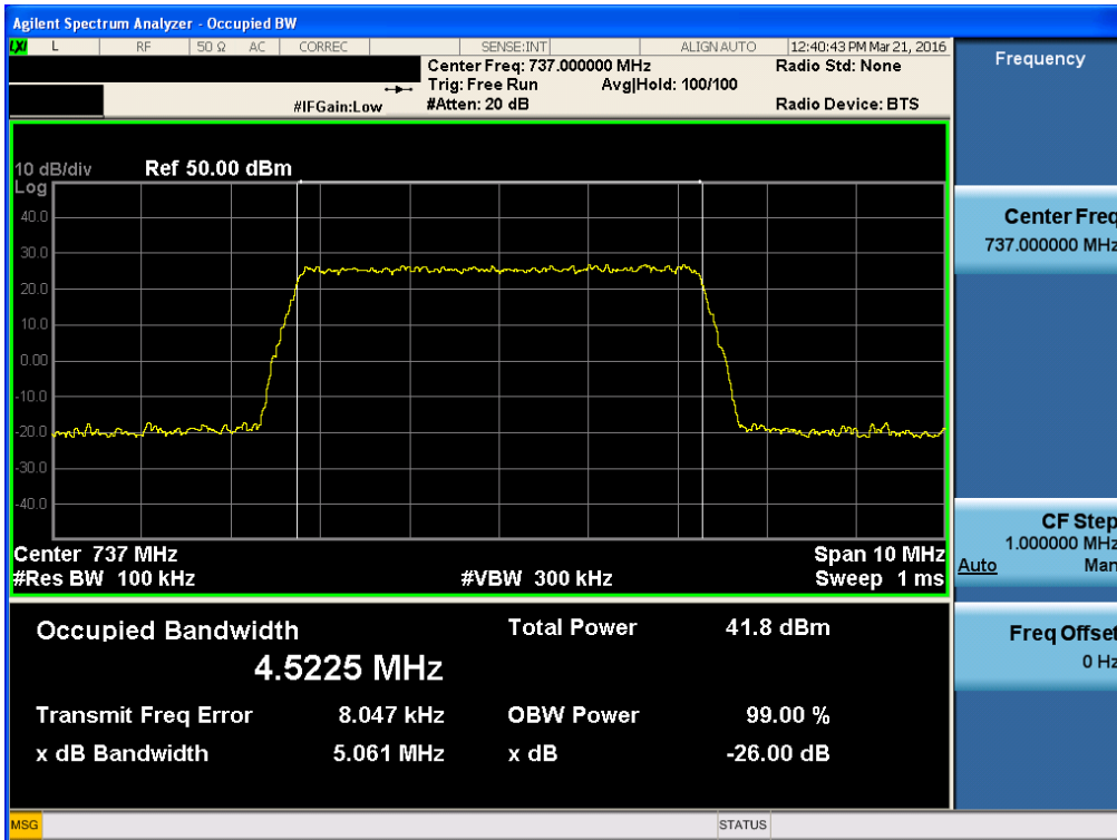
[Output Downlink Middle_AGC threshold]
