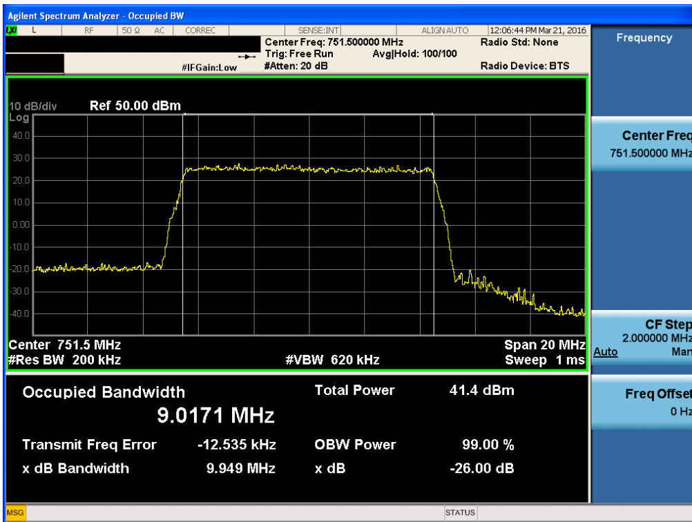
[Output Downlink Middle_ +3 dB above the threshold]
