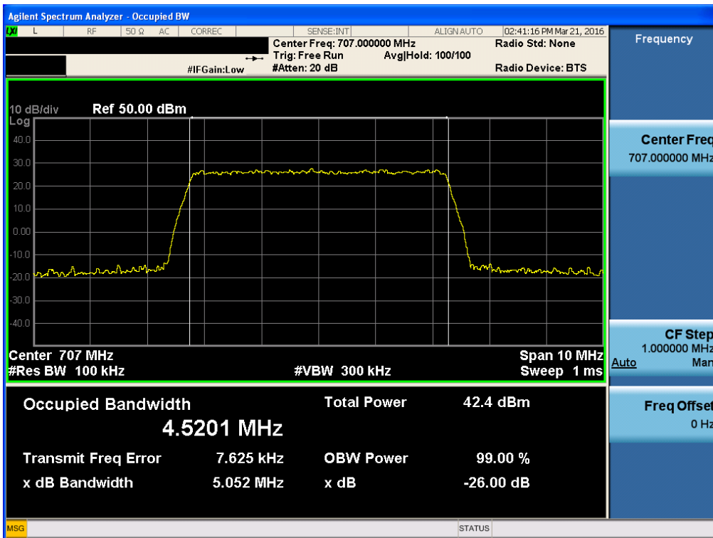
[Output Uplink Middle_ AGC threshold]
