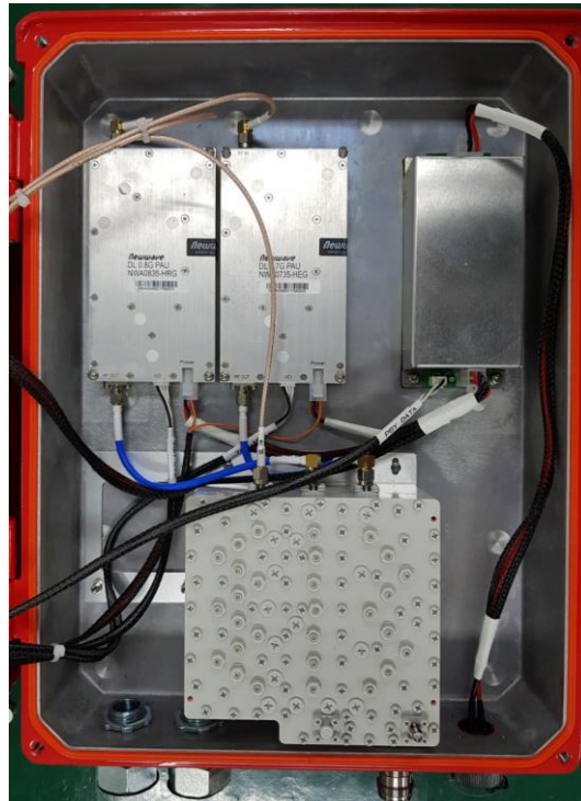
Bottom Panel
