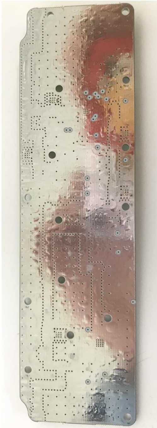
[SU RFPU BOARD UL 700 – BOTTOM]
