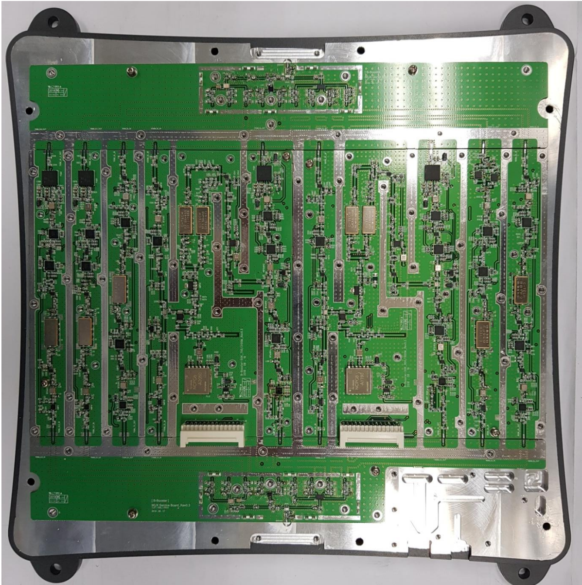
[Board - Top]
