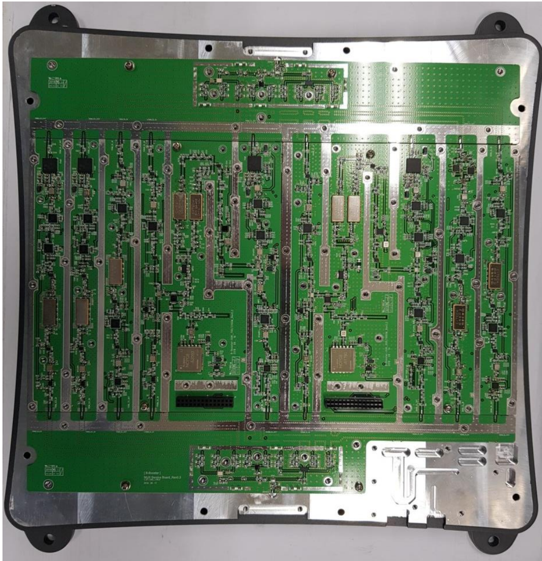
[Board - Top]
