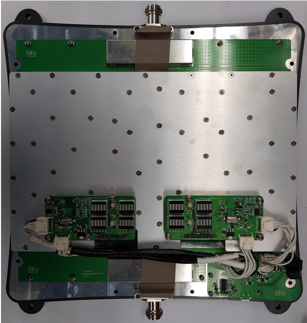
[Board - Bottom](2)
