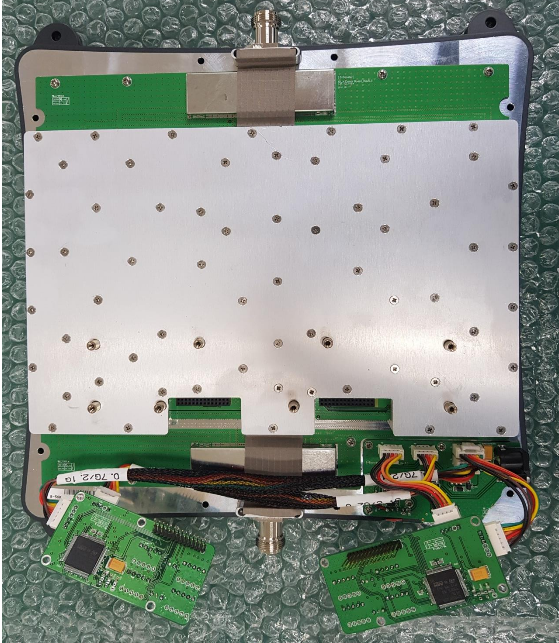
[Board - Bottom](1)
