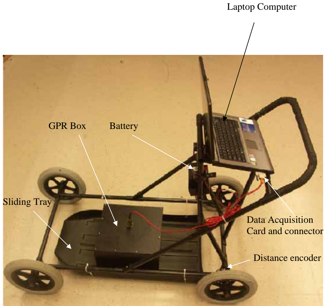
Figure 1-2 GPR system in measurement configuration
