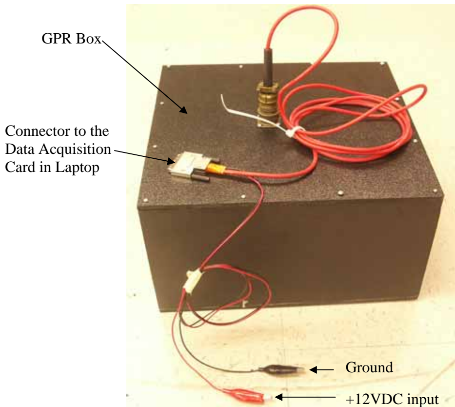
Figure 2-1 Developed GPR
