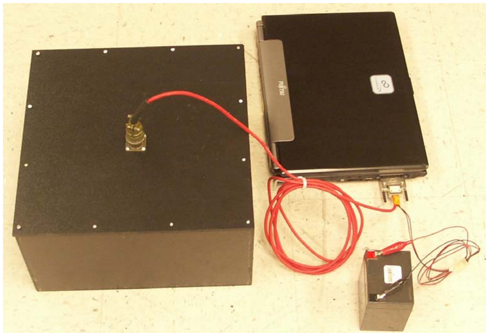
Figure 8 Electrical connection of the GPR system
