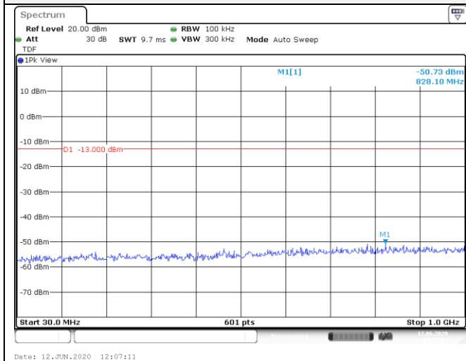
30MHz-1GHz
