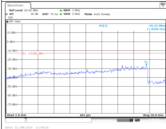
2GHz-20GHz
