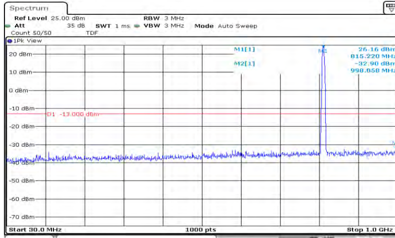
Band26-1.4MHz-QPSK-26697-6RB#0-Range1:30~1000MHz
