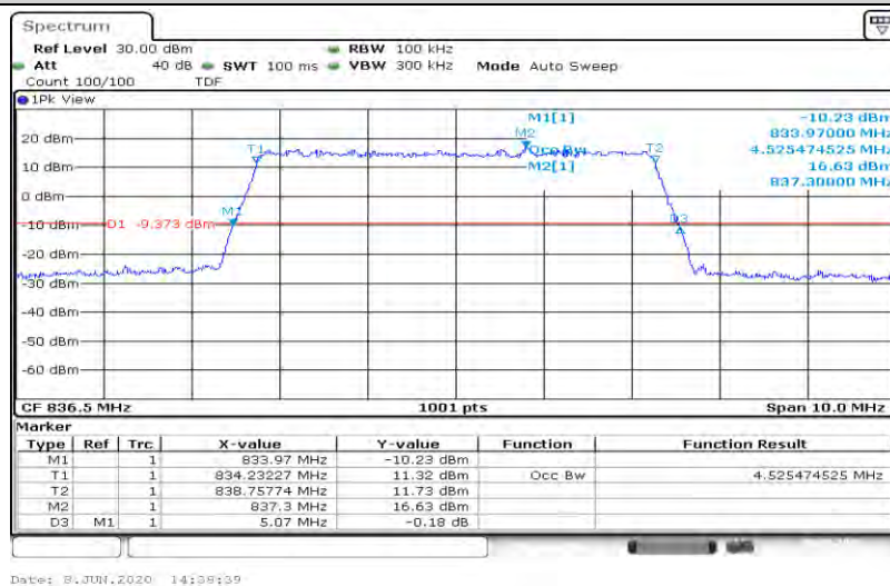
Band5-5MHz-QPSK-20625-25RB#0-4.525
