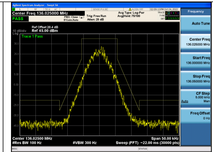
Emission Mask D@173.975MHz-10W-4FSK
