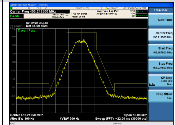
Emission Mask D@479.975MHz-10W-4FSK
