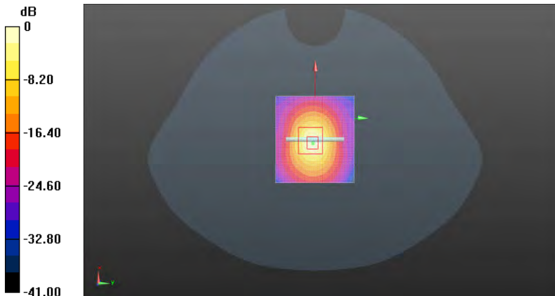
System Performance Check 5600MHz 100mW
